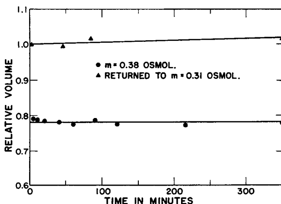
FIGURE 1 Stability and reversibility of mean cell volume at two osmolalities.
